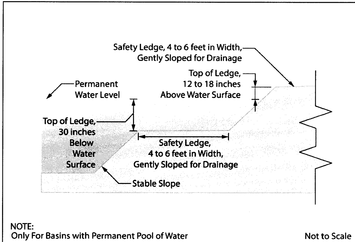
Elevation View –Basin Safety Ledge Configuration
